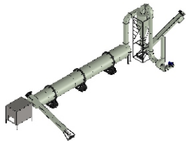
Rotary Drum Dryer upto 5000 kg/hr (Production Range)
